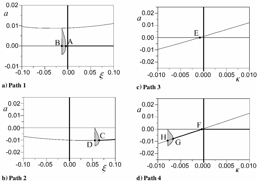
Fig. 7 Bifurcation diagrams along the path shown in Fig. 6: —, stable and —, unstable.
