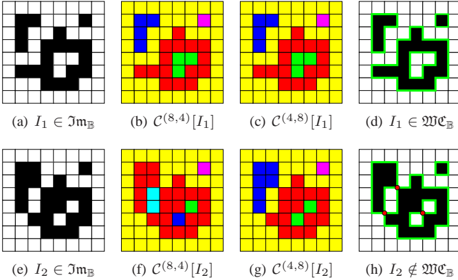
Fig. 1. (a) An image I_1 \in \mathfrak{I}\mathfrak{m}_{\mathbb{B}} . (b) The 8-connected components of \Omega = I_1^{-1}(\{1\}) and the 4-connected components of \bar{\Omega} = I_1^{-1}(\{0\}) . (c) The 4-connected components of \Omega and the 8-connected components of \bar{\Omega} . Note that I_1 has the same topological structure as a (8,4)- and as a (4,8)-image. (d) Then, I_1 can also be considered in the well-composedness model: the boundaries shared by its foreground and background regions, depicted in green, are 1-manifolds. (e) An image I_2 \in \mathfrak{I}\mathfrak{m}_{\mathbb{B}} . (f) The 8-connected components of \Omega = I_2^{-1}(\{1\}) and the 4-connected components of \bar{\Omega} = I_2^{-1}(\{0\}) . (g) The 4-connected components of \Omega and the 8-connected components of \bar{\Omega} . Note that I_2 does not have the same topological structure as a (8,4)- and as a (4,8)-image. (h) Then, I_2 cannot be considered in the well-composedness model: the boundaries shared by its foreground and background regions, depicted in green, are not 1-manifolds (see the red dots). (a,d,e,h) \Omega is depicted in black, and \bar{\Omega} in white. (b,c,f,g) For the sake of readability, each connected component is represented by a different colour.
