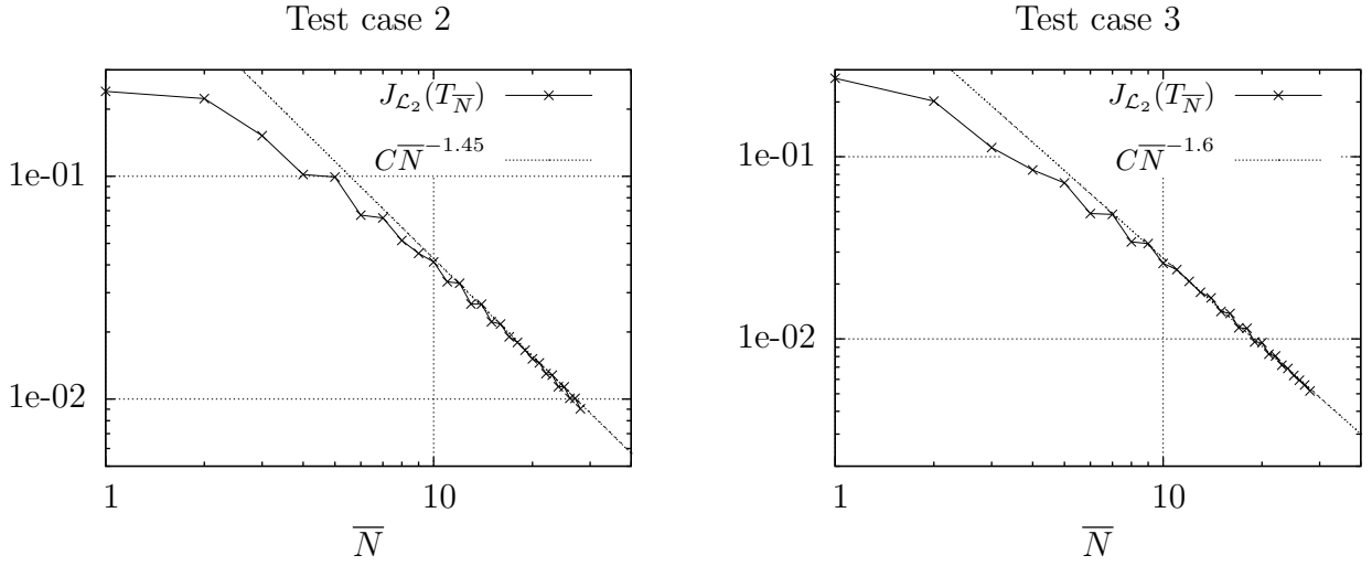
Figure 7: Convergence of J_{\mathcal{L}_2}(T_{\bar{N}}) toward 0 versus \bar{N} in bi-logarithmic scale for test cases 2 and 3.
