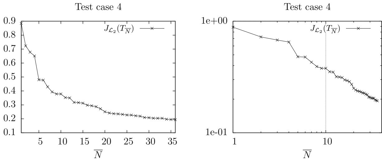
Figure 15: Convergence of J_{\mathcal{L}_2}(\bar{N}) toward zero versus the mode truncation order \bar{N} in linear scale (left) and using log-log scale (right) for test case 4 configuration.
