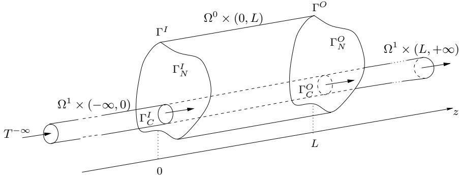
Figure 4: Exchanger coupling with one inlet and one outlet tube and with \Omega^1 = \Omega^2 studied in Sec. 2.4. On this example illustration, an adiabatic frontier \Gamma_{N}^{I,O} is added. The temperatures at infinity are homogeneous and equals to T^{\pm\infty} , T^{-\infty} is a data and T^{+\infty} is an unknown.
