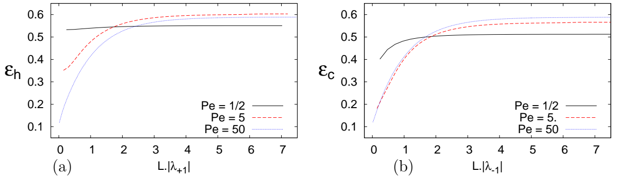
Figure 17: Same conventions as in Fig. 16 except that the results are plotted versus re-normalized length L \cdot \lambda_{\pm 1} where the first eigenvalues \lambda_{\pm 1} provide the inverse of the upstream or downstream typical longitudinal length variations.
