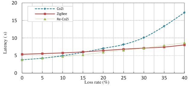
Figure 4 – Latency versus packet loss rate
