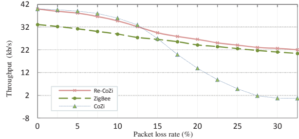
Figure 5 – Throughput versus packet loss rate
