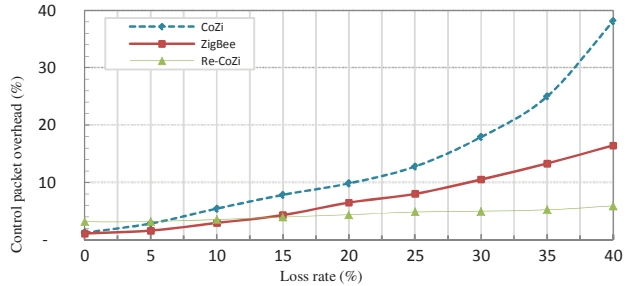
Figure 6 – Control packet overhead
