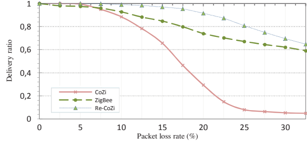
Figure 3 – Delivery ratio versus packet loss rate
