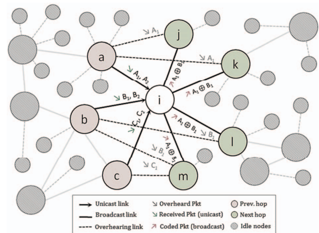
Figure 1 - ZigBee overhearing example
