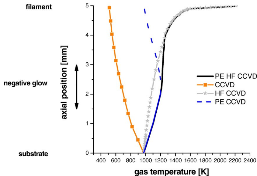
Fig. 2. Temperature profiles versus axial position in the CVD chamber. Substrate temperature is fixed at 973 K. Ordinate origin is the sample position and the lower filament is set at 5 mm above the sample.
