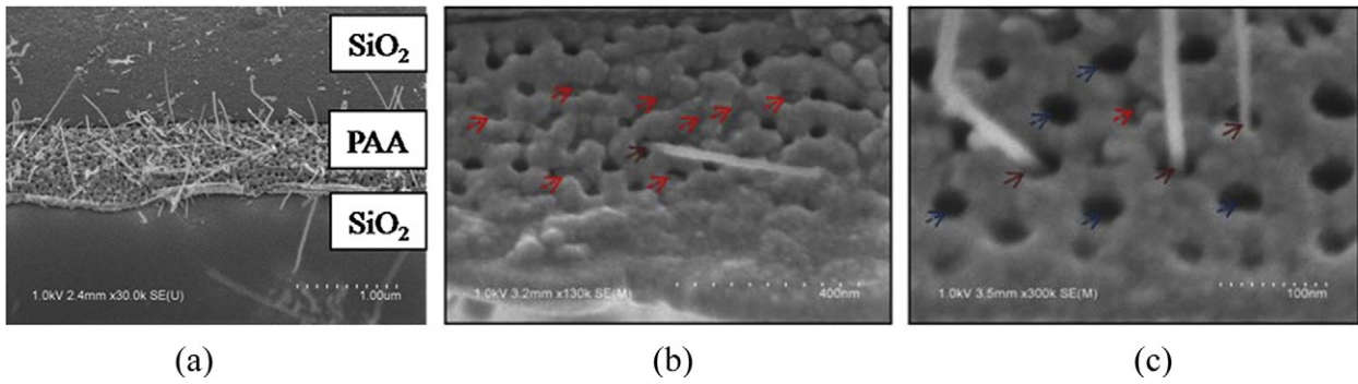
Fig. 6. Various SEM pictures of Si NWs grown in porous lateral templates. (a): View of a membrane after growth with H + . The NWs are clearly seen emerging from some of the pores. (b): Another membrane after growth without H + (the W filament was not turned on); the red arrows point to those pores blocked by amorphous Si deposition and the brown one to an emerging NW. (c): Close up of the picture shown in (a). The red and brown arrows have the same meaning as in (b); the blue arrows indicate partially filled or empty pores.
