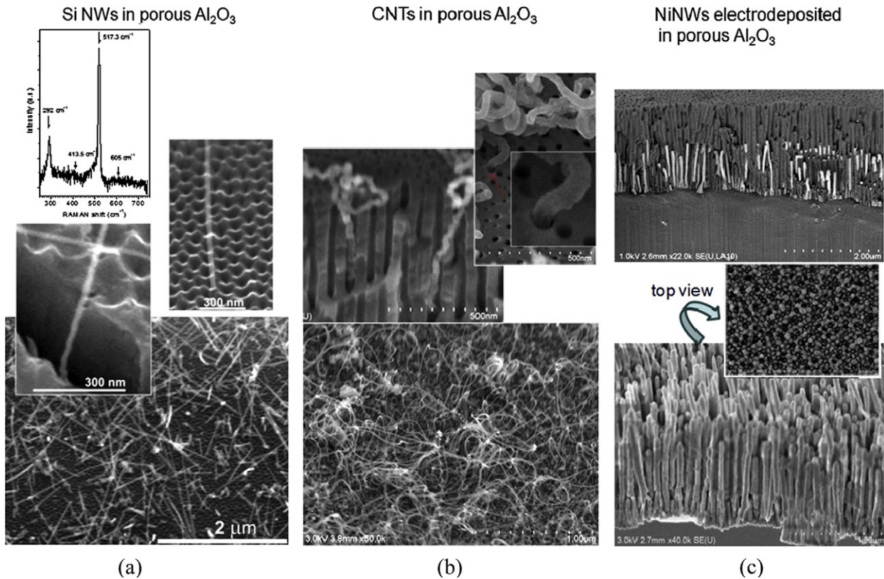
Fig. 2. Various nanostructures grown inside vertical porous alumina templates. (a): Different SEM views of Si NWs grown from electrodeposited Cu catalysts. From bottom to top: (i) surface of the membrane after VLS growth; for easy observation, the growth time has been purposely made longer, which results in NWs growing out of the membrane, (ii) detail of a NW emerging from a pore, (iii) the membrane has been broken in order to check that NW nucleation occurred at the bottom of the pores, where the Cu nanoparticles are electrodeposited, (iv) Raman spectrum of the nanowires evidencing their good crystalline quality. (b): Different views of CNTs grown from electrodeposited Ni catalysts. From bottom to top: (i) surface of the membrane after VLS growth, (ii) cross section of a membrane showing CNTs inside it, (iii) details of CNTs emerging from the membrane, with a close view on one CNT in inset ( \sim 40 nm diameter). (c): Ni NWs grown by electrodeposition from a mixture of \text{NiSO}_4 , \text{NiCl}_2 and \text{H}_3\text{BO}_3 (Watts bath). The membrane has been selectively etched in the bottom picture, in order to reveal the Ni NWs which were originally inside the pores.
