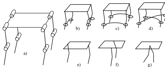
Figure 1: Description of the robot and studied gaits.
