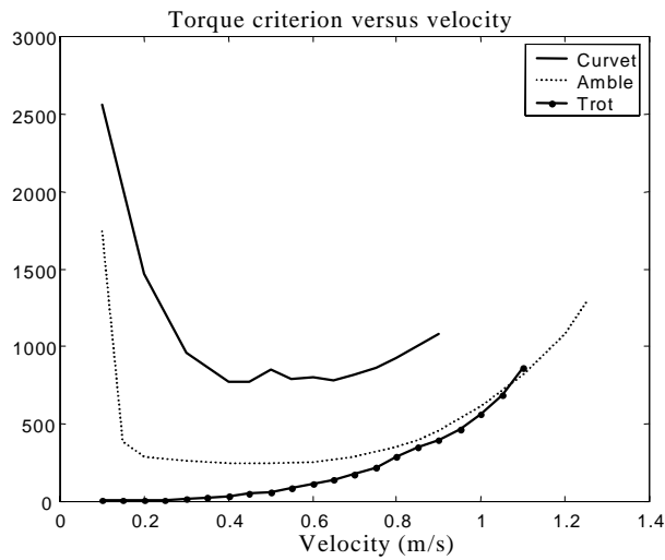
Figure 13: Torque cost criterion versus velocity for the three gaits.
