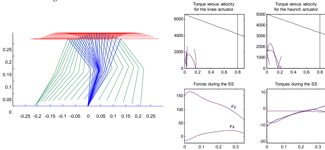
Figure 11: Trot simulation results with minimization of the torque cost.
