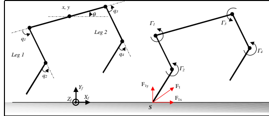
Figure 2: Generalized coordinates and forces of the quadruped for curvet .
