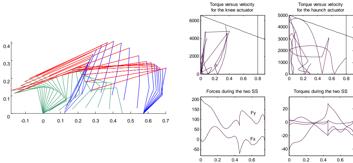
Figure 9: Curvet simulation results with minimization of the torque cost.
