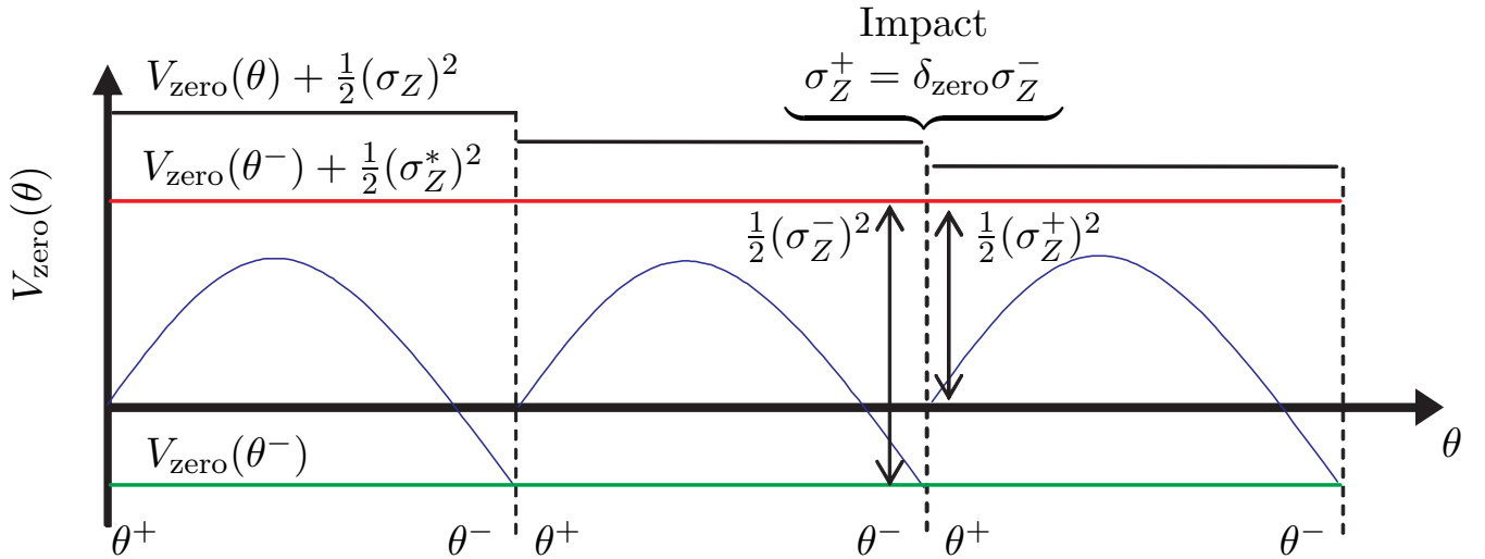
Fig. 14. A Qualitative Look at Stability Through Energy. The zero dynamics is Lagrangian, and thus throughout the single support phase, the corresponding total energy V_{\text{zero}}(\theta) + \frac{1}{2}\sigma_Z^2 is constant. At impact, the change in total energy depends on the angular momentum through \delta_{\text{zero}}\sigma_Z^- and the potential energy through V_{\text{zero}}(\theta^-) . The total energy corresponding to the periodic orbit is V_{\text{zero}}(\theta^-) + \frac{1}{2}(\sigma_Z^*)^2 . Convergence to this total energy level occurs if the angular momentum decreases during impact, namely, \delta_{\text{zero}} < 1 . From the expression for the existence of a periodic orbit, \delta_{\text{zero}} < 1 is equivalent to V_{\text{zero}}(\theta^-) < 0 .
