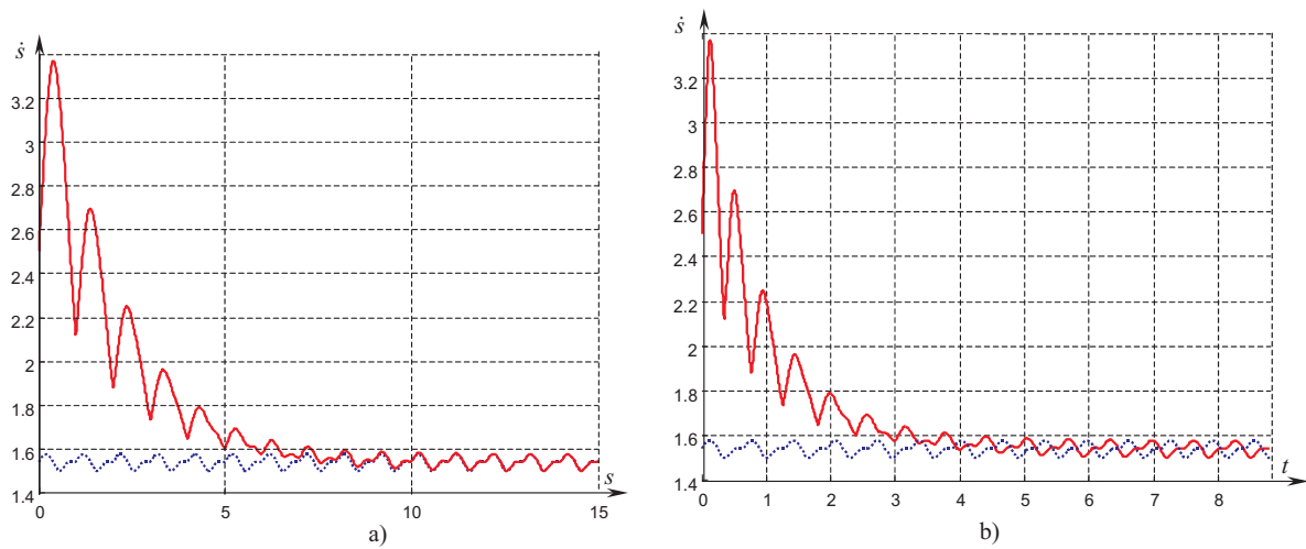
Fig. 9. The proposed control ensures orbital stability: a) evolution of velocity \dot{s}(s) (solid line), and of cyclic velocity \dot{s}_c(s) (dotted line) for 15 steps, b) evolution of velocity \dot{s}(t) (solid line), and of cyclic velocity \dot{s}_c(t) (dotted line) for 15 steps.
