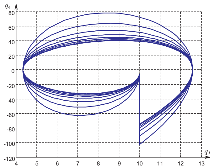
Fig. 10. Evolution in degrees of angle q_5 in its phase plane.
