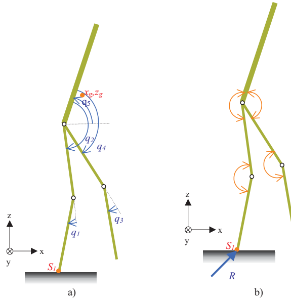
Fig. 1. The studied biped: a) generalized coordinates, b) applied torques and ground reaction.
