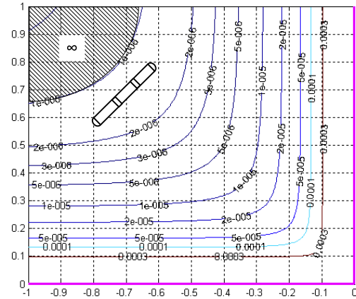
(b) The contours of the iso-current I_s for a sensor tilted of \alpha = 45^\circ .
