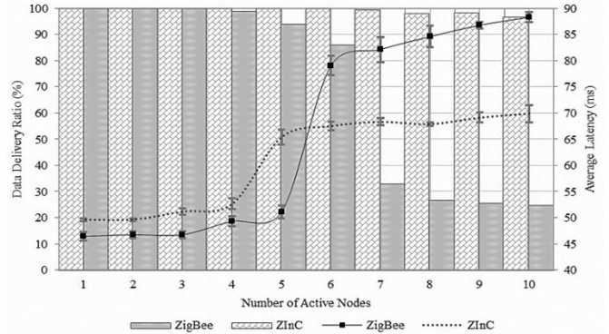
Figure 7 – Latency vs. Number of Sources vs. Data Delivery Ratio
