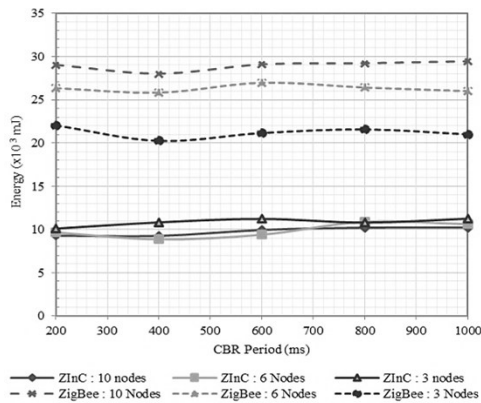
Figure 9 – Energy Consumption vs. CBR Bitrate
