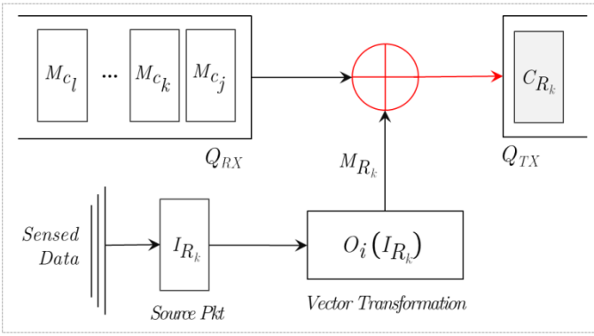
Figure 2 – Index-coding phases at an intermediate ZigBee router R_k
