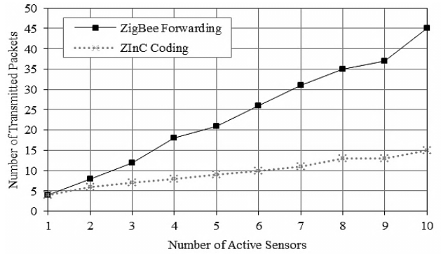
Figure 6 – Average Number of Transmissions vs. Number of Sources
