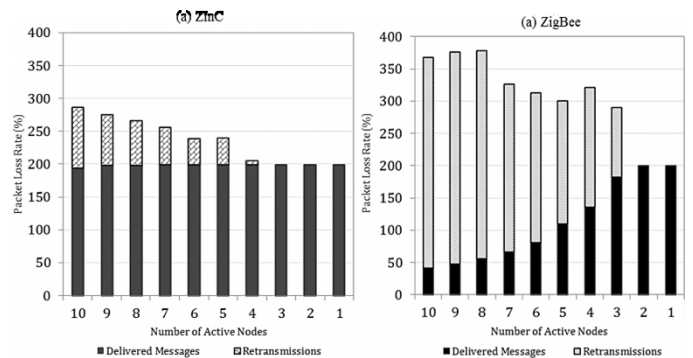
Figure 8 – Number of Sources vs. Number of Delivered Packets
