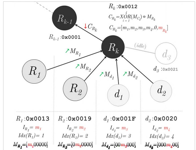
Figure 4 – Index-Coding Illustration
