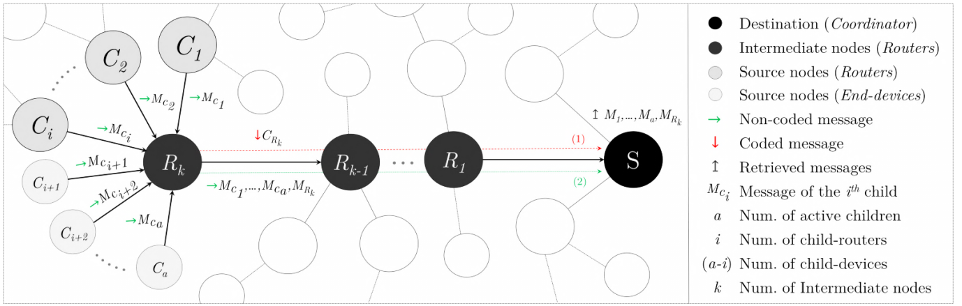
Figure 1 – Nodes C_1, \dots, C_a send their data to S via a k hops route either with ZigBee routing (in green) or via ZInC coding (in red)
