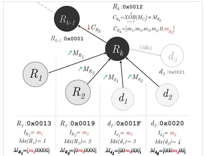
Figure 4 – Index-Coding Illustration
