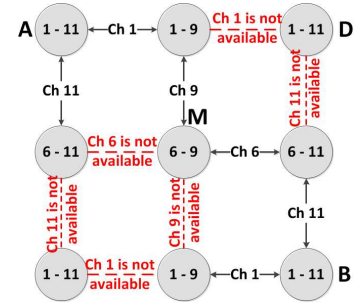
Fig. 5. Tiered channel allocation
