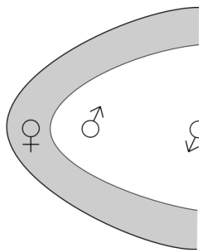
Parabole
