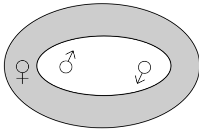
Ellipse
