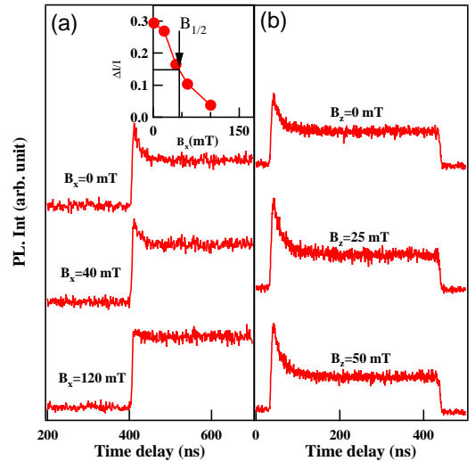
FIG. 4: (Color online) Mn spin transient as a function of a magnetic field applied in-plane (a) and out-of-plane (b). Inset: transverse field dependence of the transient amplitude \Delta I/I (see Fig. 1). B_{1/2} is the half width at half maximum.
