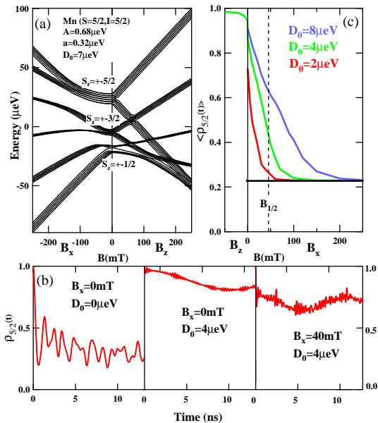
FIG. 5: (Color online) (a) Magnetic field dependence of the fine structure of the Mn spin with out-of-plane (right) and in-plane (left) field, calculated with A = 0.68 \mu\text{eV} , D_0 = 7 \mu\text{eV} and a crystal field parameter a = 0.32 \mu\text{eV} . (b) Time evolution of \rho_{+5/2}(t) calculated for different values of D_0 and B_x with \rho_{+5/2}(0) = 1 . (c) Time average value of \rho_{+5/2}(t) versus B_x for different values of D_0 ( T_2 = \infty ). The B_{1/2} found experimentally is indicated with a dotted line.
