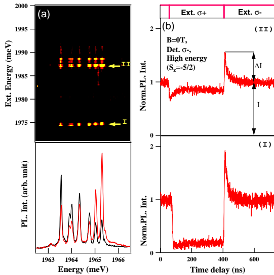
FIG. 1: (Color online) (a) PL and PL excitation of a Mn-doped QD at B = 0 T and T = 5 K. The PL is detected in circular polarization under an alternate \sigma^-/\sigma^+ excitation at two different wavelengths into the same set of excited states: 1987.0 meV (black) and 1987.4 meV (red). (b) PL transient under polarization switching at B = 0 T. The PL is detected on the high energy line of X-Mn in \sigma^- polarization (Mn spin S_z = -5/2 ). Transient (I) (resp. (II)) was observed under resonant excitation at 1975 meV (resp. 1987 meV)
