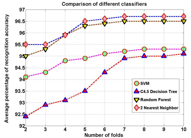
Fig. 2. Evolution of the achieved average recognition accuracy for the six universal facial expressions with the increasing number of folds for the k -fold cross validation technique.
