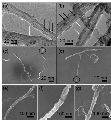
FIG. 1. TEM images of (a) MWNT-ferritin and (b) MWNT-FeO x NP conjugates, showing CNTs (white arrows) decorated with metal particles (black arrows). SEM images of individual regrowth events from (c) MWNT-ferritin and (d) MWNT-FeO x NP conjugates. Circles show the probable location of the catalyst particle. SEM images showing the primary MWNTs after CVD growth in (e) MWNT-ferritin, (f) MWNT-FeO x NP, and (g) MWNT with DEP deposited FeO x NP samples.
