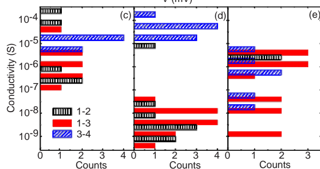
FIG. 2. (Color online) (a) SEM image and (b) I - V characteristics of an electrically connected CNT junction obtained from MWNT-FeO x NP conjugates. [(c)–(e)] Histograms of conductances (see Ref. 20) for (c) MWNT-ferritin, (d) MWNT-FeO x NP conjugate, and (e) DEP deposited MWNT and FeO x NP samples. The primary CNT is measured between electrodes 1 and 2, the secondary CNT between 3 and 4 and the junction between 2 and 3.
