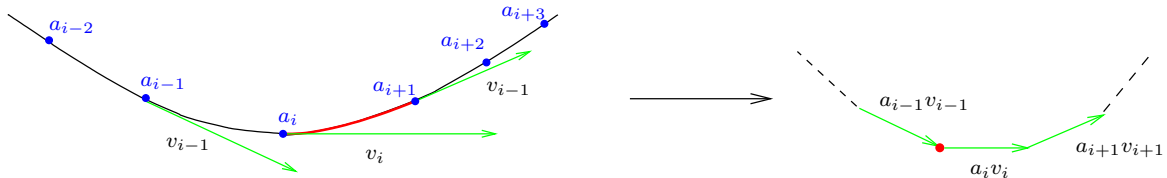
Figure 9: Proof of Theorem 4.11 in the d = 1 case. The point on the right hand picture is chosen arbitrarily. v_k is a unit vector orthogonal to the point of \mathbb{H}^1 of weight a_k .
