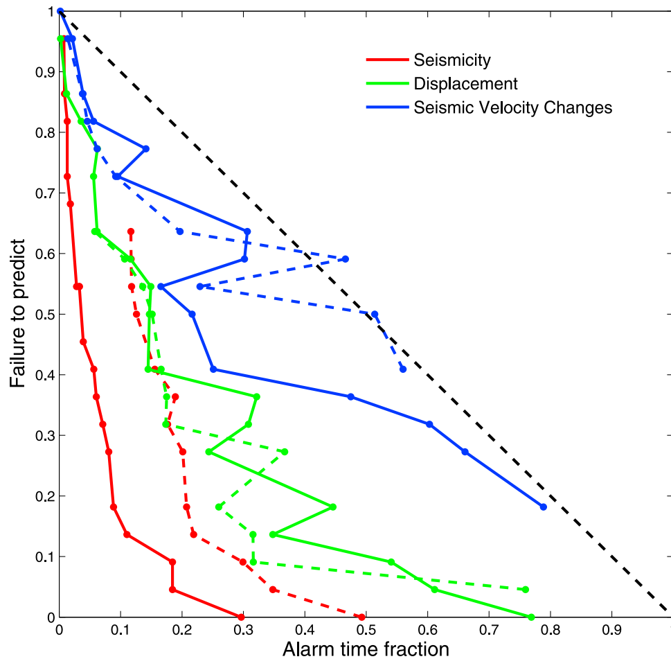
Figure 13. Envelopes of the prediction outputs in the failure to predict versus alarm time fraction diagram for the 3 forerunners, when minimizing equation (2). Plain lines are the rate values, dotted lines are the cumulative values.
