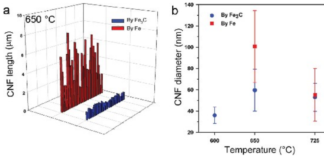
Figure 4. Effect of Fe and \text{Fe}_3\text{C} on the growth of CNFs. (a) Plots of the measured lengths of CNFs catalyzed by Fe and \text{Fe}_3\text{C} at 650 °C. The length of CNFs was measured by TEM on randomly picked specimens. (b) Spreading of diameter values for CNFs/CNTs catalyzed by Fe and \text{Fe}_3\text{C} as a function of growth temperatures. Both the averaged values and standard error bars are shown.
