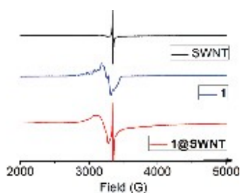
Figure 2. Comparison of EPR spectra of purified nanotubes (powder) (black curve), free 1 in CH 2 Cl 2 /DMF (1:1) solution (blue curve), and 1 @SWNT (powder) obtained after filtration and extensive washing (red curve).
