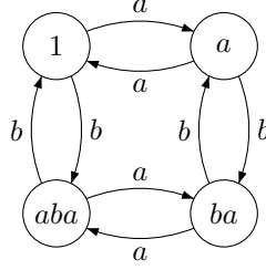
Figure 6.9: The associated coset automaton.
