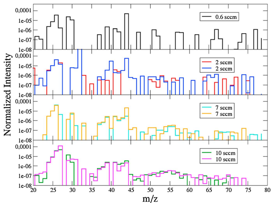
Figure 10. Difference between the MSs of the initial state and the state after ~1 h irradiation obtained for various gas flows in the APSIS reactor (and HP conditions in the MS).
