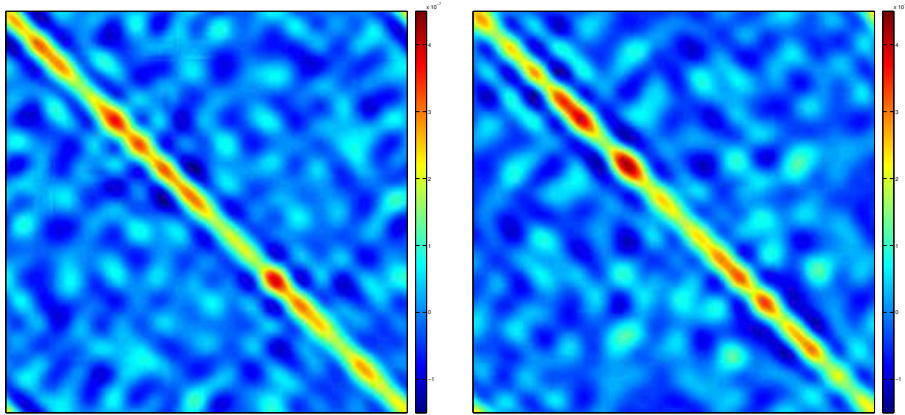
Figure 6. Visualization (with 50 members) of the covariance matrix values corresponding to the central line at t = 99 left: ETKF, right: WETKF. The significant covariance length-scale is about 15 \times \Delta x large for both filters
