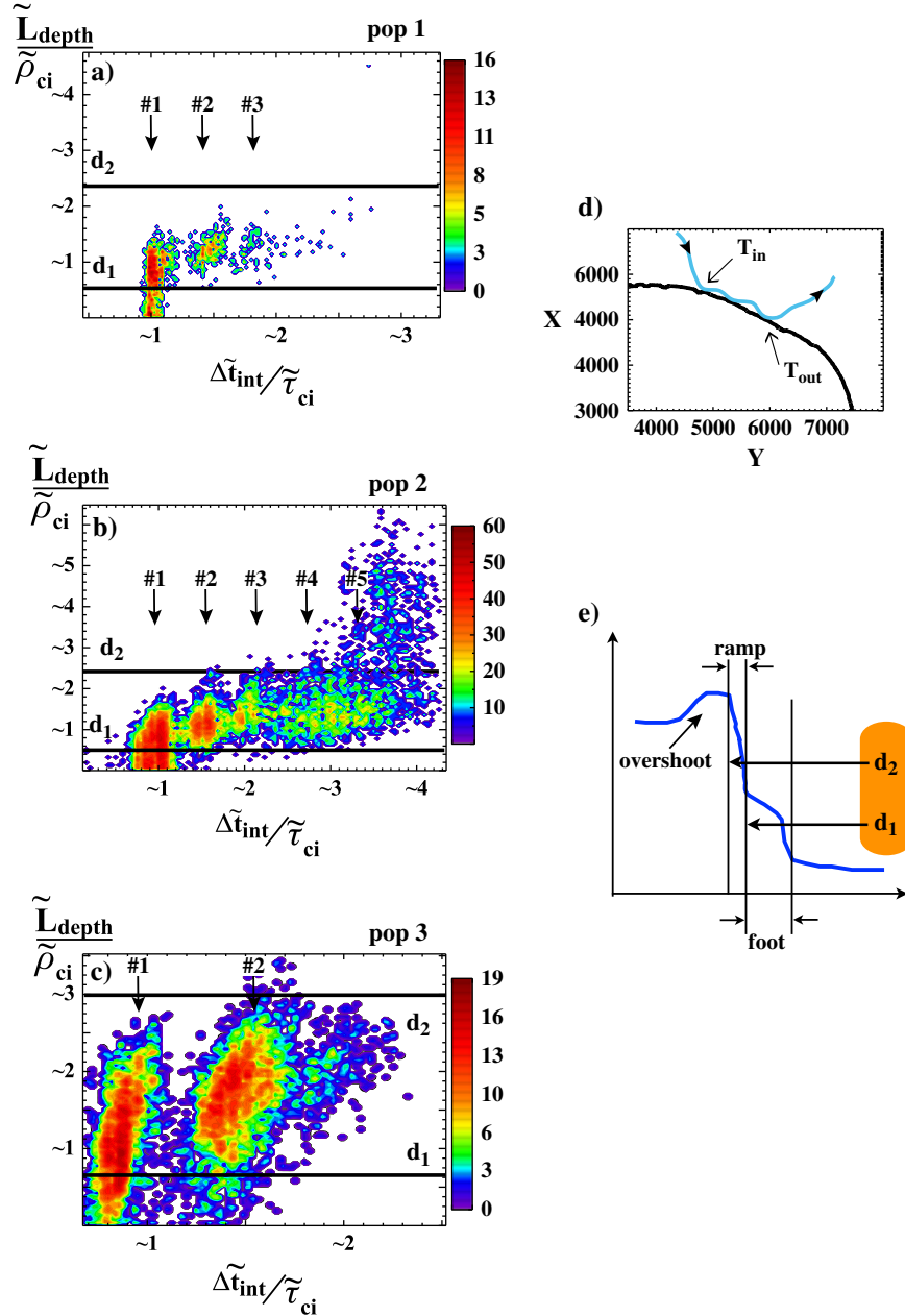
Figure 5. (a–c) show the penetration depth \tilde{L}_{\text{depth}} of incoming ions through the shock front (normalized to the upstream ion gyroradius \tilde{\rho}_{ci} ) before being reflected back upstream versus the total interaction time \Delta\tilde{t}_{\text{int}} with the shock front (normalized to the upstream ion gyroperiod \tilde{\tau}_{ci} ) for each population 1, 2, and 3 defined in Figure 2, respectively. On each plot, the different “burst” have been labeled #1, #2, . . . The interaction time \Delta\tilde{t}_{\text{int}} is illustrated in (d) where \Delta\tilde{t}_{\text{int}} = \tilde{T}_{\text{out}} - \tilde{T}_{\text{in}} . Two distinct characteristic lengths, d_1 and d_2 , represent the distance of penetration into the shock to reach the ramp and the overshoot and are sketched in (e).
