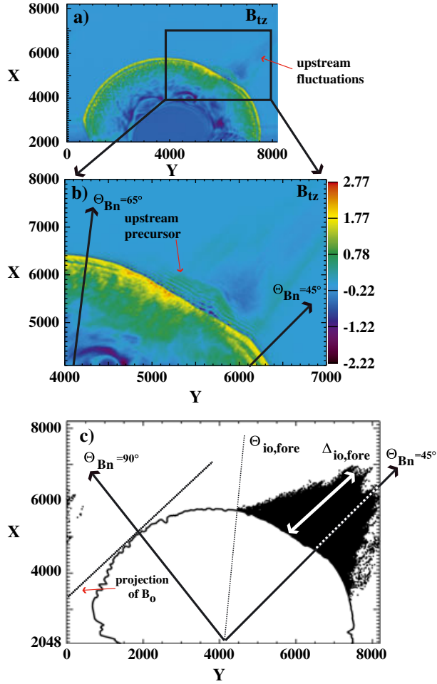
Figure 1. View of the developed curved shock within the simulation plane X-Y plotted at time \tilde{t} = 5.4\tilde{\tau}_{ci} where \tilde{\tau}_{ci} is the upstream cyclotron ion period. (a) shows the main magnetic field component \tilde{B}_{tz} . The ambient magnetostatic field \tilde{B}_o (representing the interplanetary magnetic field) is imposed along a direction of 45^\circ outside the simulation plane. Then the whole angular range of curved shock is lying within 45^\circ \leq \theta_{Bn} \leq 90^\circ . (b) is an enlarged view of the 45^\circ \leq \theta_{Bn} \leq 65^\circ region showing details of the upstream magnetic field. (c) plots the ions locations within the ion foreshock where backstreaming ions satisfied the criteria detailed in the text. For reference, straight arrows represent the normal of the shock front at \theta_{Bn} = 90^\circ and \theta_{Bn} = 45^\circ . The dotted line represents the projection of the upstream field \tilde{B}_o into the simulation plane. Two parameters have been also reported: (i) \theta_{io,fore} ( \approx 66^\circ ) the leading edge angle of the ions foreshock and (ii) \Delta_{io,fore} the extend of the ion foreshock measured from the curved front at the end of our simulation.
