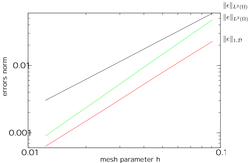
FIGURE 2. Errors for the velocity and the pressure obtained with squared control volumes.
