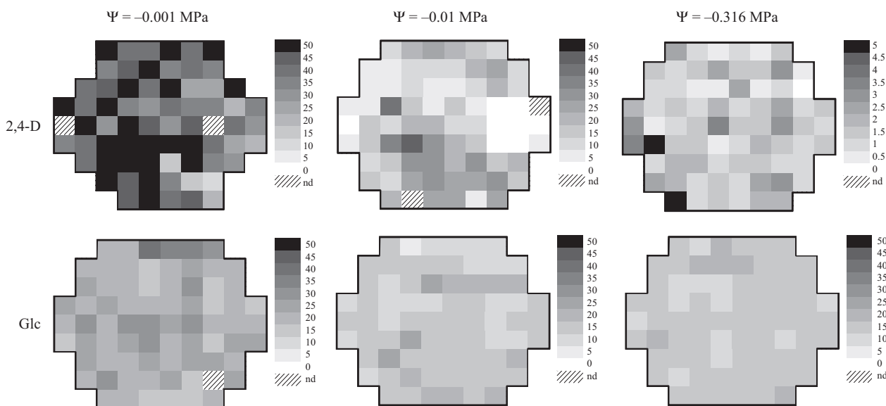
Fig. 2. Spatial distribution of 2,4-D (top row) and glucose (bottom row) mineralization (represented as % of added substrates) at different matric potentials ( \Psi = -0.001 , -0.01 and -0.316 MPa). Each square represents the mineralization in one spatially referenced soil cube. Note that the scale for the 2,4-D mineralization at \Psi = -0.316 MPa is reduced to allow visualization of the spatial heterogeneity. (nd: not determined).
