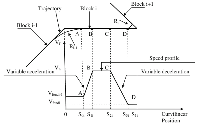
Fig. 6 Correspondence between the trajectory and the speed profile
