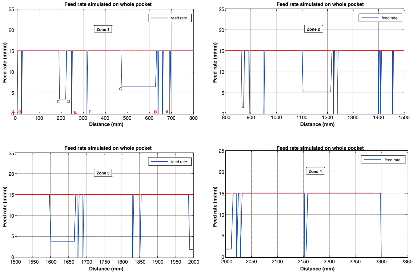
Fig. 15 Simulated feed rate profile (static look ahead) detailed over four areas
