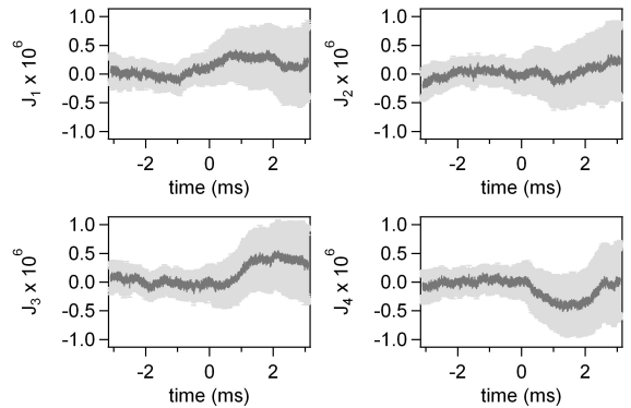
Figure 7. Time evolution of J_1 , J_2 , J_3 and J_4 (dark grey curve) and their uncertainties at 3\sigma confidence level (light grey).
