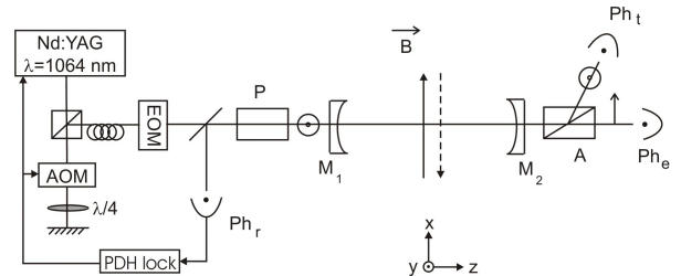
Figure 2. Experimental setup. EOM, electro-optic modulator; AOM, acousto-optic modulator; PDH, Pound-Drever-Hall; \text{Ph}_r , photodiode; P, polarizer; A, analyzer. See text for more details.
