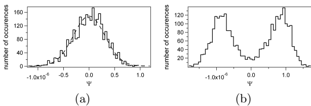
Figure 5. Typical histogram of \Psi(t) before the magnetic pulse. a) The histogram can be fitted by a gaussian function (dashed curve) : the shot is selected. b) Rejected shot.
