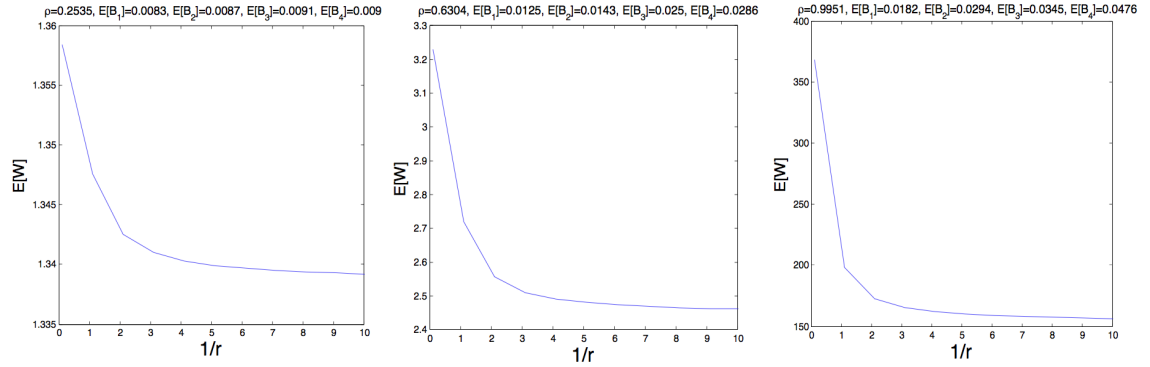
Figure 2: The mean waiting time for four classes of customers in the system, K=4 , under DROS for the loads \rho = 0.2535, \rho = 0.6304 and \rho = 0.9951 , respectively. The horizontal axis corresponds to \frac{1}{r} = \frac{p_j}{p_{j+1}}, j = 1, \dots, K-1 .
