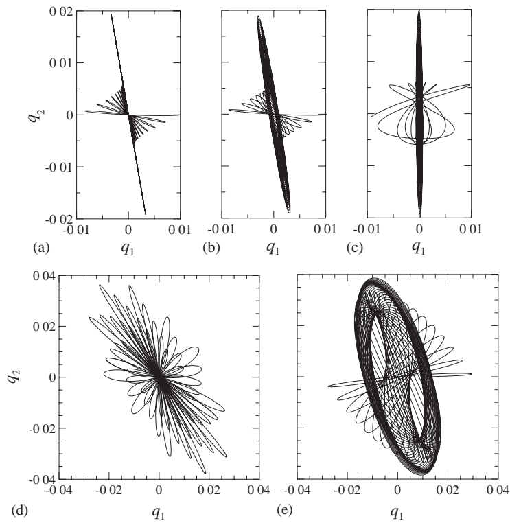
Fig. 13. Galloping motions: RMP cross section ( c_d = 1.07 , c_l = 0.60 , c'_d = 1.06 , c'_l = 1.39 ), (a) \sigma = 0 , \mu_{cr} = 0.0266 , \mu = 0.045 , (b) \sigma = 0.02 , \mu_{cr} = 0.0287 , \mu = 0.045 , (c) \sigma = 0.5 , \mu_{cr} = 0.0435 , \mu = 0.07 ; NDT cross section (point P_3 : c_d = 0.41 , c_l = 1.01 , c'_d = 0 , c'_l = 1.49 ), (d) \sigma = 0 , \mu_{cr} = 0.1077 , \mu = 0.18 , (e) \sigma = 0.02 , \mu_{cr} = 0.0186 , \mu = 0.03 .
