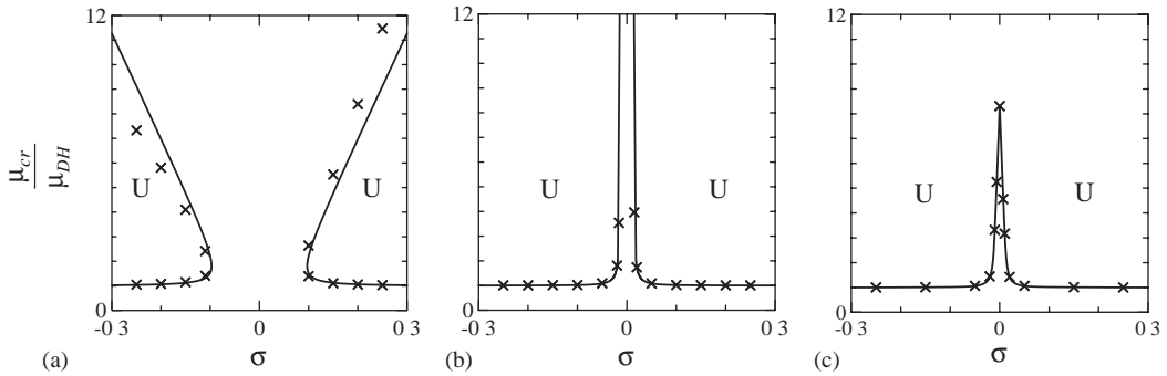
Fig. 10. Critical wind velocity vs. detuning for the NDT cross section family at points P_1, P_2, P_3 of Fig. 9: c_l = 1.01 , c'_d = 0 , c'_l = 1.49 ; (a) c_d = 1.01 , (b) c_d = c'_l/3 , (c) c_d = 0.41 ; U unstable regions; \times numerical values.
