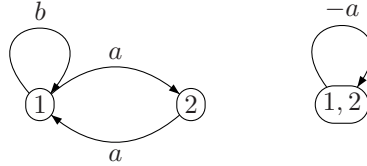
Figure 5: The even automaton
