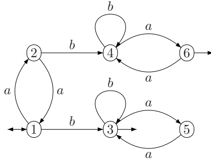
Figure 6: The minimal automaton of X .
