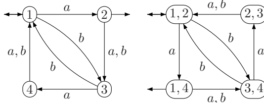
Figure 3: The automata \mathcal{A} and \tilde{\mathcal{A}} .
