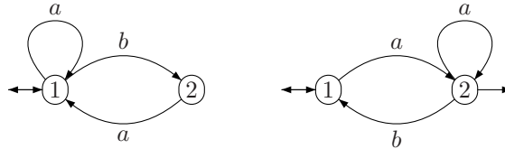
Figure 2: The minimal automata of X^* and \tilde{X}^* .
