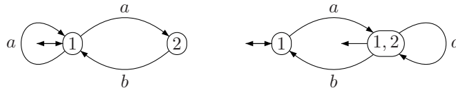
Figure 1: A nondeterministic automaton and the result of the accessible set construction.
