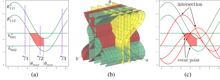
Fig. 6. (a) Progression of the cut \gamma in the cross-section \mathcal{R}_{\mathcal{H}} of FRTS \mathcal{R} on the plane (a, \theta) . The initial cut is \gamma_1 = (h_{111}^+, h_{112}^+, h_{001}^+, h_{002}^-) ; when it goes in \mathcal{R}_{\mathcal{H}} it has become \gamma_2 = (h_{001}^+, h_{111}^+, h_{002}^-, h_{112}^-) ; when it goes out of \mathcal{R}_{\mathcal{H}} it becomes \gamma_3 = (h_{111}^+, h_{112}^+, h_{001}^+, h_{002}^-) . (b) Example of tipping surfaces (in red) passing \mathcal{R} in the parameter space (a, b, \theta) and (c) its cross-section \mathcal{R}_{\mathcal{H}} on the plane (a, \theta) .
