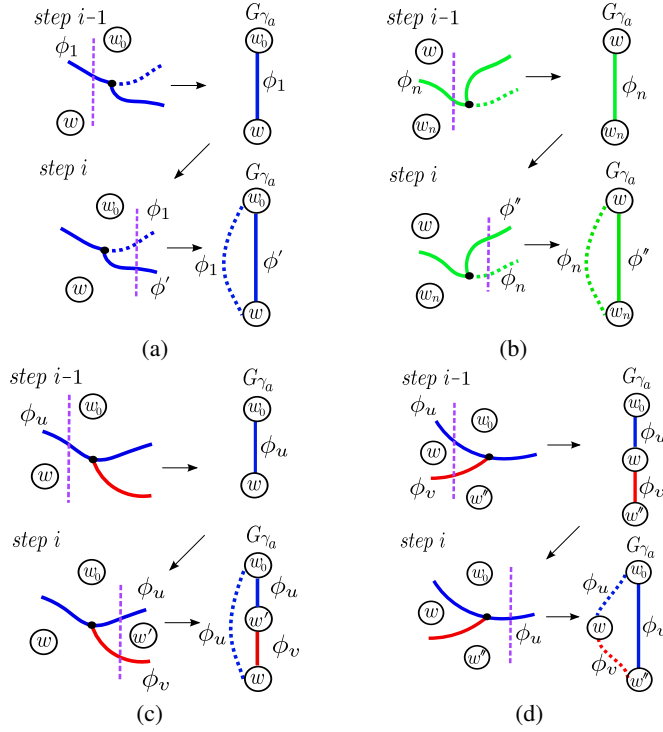
Fig. 10. Illustrations of elementary steps –update \gamma and generate its graph G_{\gamma} – for a tipping curve changing (a) an upper or (b) a lower boundary, and going (c) in or (d) out of an upper boundary.
