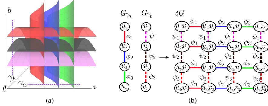
Fig. 5. Construction of a partial graph \delta G by combining two graphs G_{\gamma_a} and G_{\gamma_b} .
