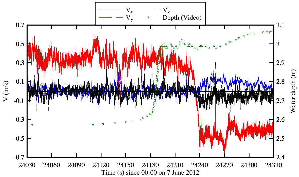
Fig. 6 - Details of the time variations of the water depth and turbulent velocity components in the tidal bore of the Garonne River on 7 June 2012
