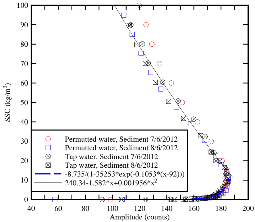
Fig. 8 - Relationship between suspended sediment concentration and acoustic signal amplitude with the sediment samples collected at Arcins - Comparison between the data and Equations (3) and (4)
