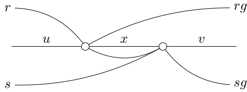
Figure 6: The interpretations \alpha_r and \alpha_s are independent. ■
