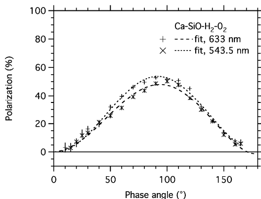
Figure 3: Polarimetric phase curves for the Ca-SiO smoke showing maximum polarization ( 54 \pm 2 ) % in red light at a phase angle of ( 95 \pm 5 )° and ( 48 \pm 2 ) % in green light at a phase angle of ( 93 \pm 5 )°.
