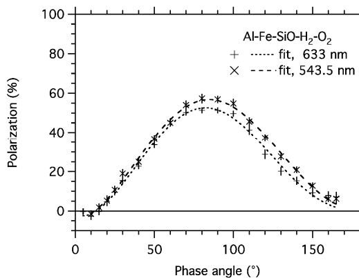
Figure 4: Polarimetric phase curves for the Al-Fe-SiO smoke showing maximum polarization ( 52 \pm 2 ) % in red light at a phase angle of ( 86 \pm 5 )° and ( 57 \pm 2 ) % in green light at a phase angle of ( 88 \pm 5 )°.
