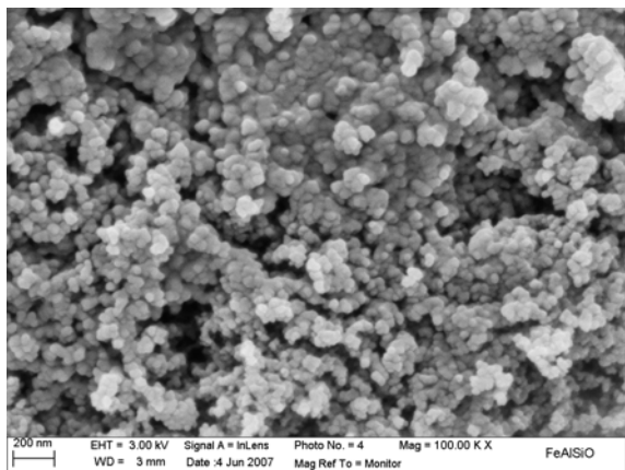
Figure 2: SEM image of the porous Al-Fe-SiO smoke that is dominated by a matrix of small grains.
