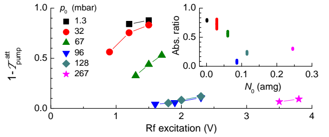
Figure 11: Fraction of light power absorbed from a low-power pump beam at M=0 with the f_2^- line at 4.7 T. Main plot : Variation with rf excitation and cell content (legend: see Fig. 9a). Inset : Same data sets, scaled to the values computed for a narrow beam (from the data in Fig. 10, see text); the bar symbols extend from min. to max. values.
