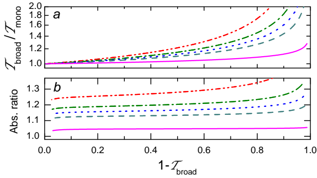
Figure 26: Broadband light transmittance \mathcal{T}_{\text{broad}} expected for a narrow beam with \mathcal{L}=1 GHz Gaussian bandwidth (1.7 GHz FWHM, similar to \bar{\omega}_{\text{G}} ). Results are obtained using Eq. (C.11) and \mathcal{T}_{\text{mono}} as input variable and referenced to the monochromatic light case [4.7 T, A_2 – B_9 line]. a : Transmittance ratio; semi-log plot. b : Absorbance ratio -\ln \mathcal{T}_{\text{broad}}/(-\ln \mathcal{T}_{\text{mono}}) . From top to bottom: 0.03 (red dash-dot-dot), 0.06 (green dash-dot), 0.09 (blue dot), 0.12 (dark cyan dash), and 0.25 amg (magenta solid).
