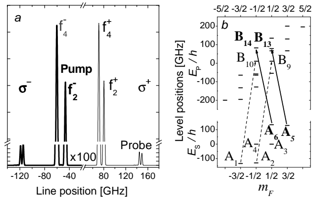
Figure 3: Hfs of the 2^3\text{S} – 2^3\text{P} transition at 4.7 T [15]. a : Absorption spectra computed at 300 K (no pressure broadening). Left, thick line: \sigma^- ; right, thin line: \sigma^+ ; horiz. axis: frequency shifts from C_1 line at 0 T. The strong f_2^- line labeled “pump” is used for OP, the weak lines of the \sigma^+ doublet labeled “probe” for detection. b : Energy diagram of 2^3\text{S} and 2^3\text{P} states (vert. axes: E_S , resp. E_P , in frequency units; ref.: 2^3\text{P}_2 energy at 0 T). The pump (resp. probe) laser simultaneously (resp. sequentially) addresses the sublevels connected by the solid (resp. dashed) arrows.
