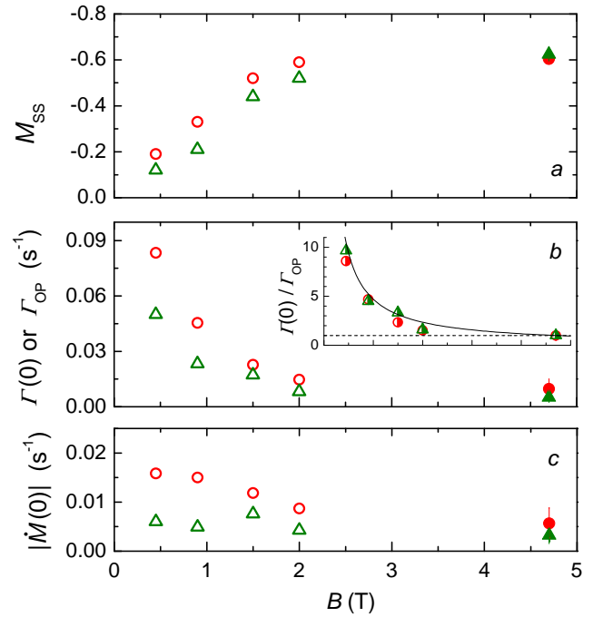
Figure 17: Comparison of MEOP results at 4.7 T (this work; solid symbols: average values in the rf plasmas, bars: spans) and at lower field ( B = 0.45\text{--}2 T, Table 2 in Ref. [13]; open symbols) for moderate density [0.03 amg: red circles, 0.06 amg: green up triangles]. a : Steady-state polarization M_{\text{SS}} . b : Build-up rates \Gamma_{\text{OP}} (constant value, 4.7 T) and \Gamma(0) (initial value, [13]; see Eq. 28). Inset : Data set ratio \Gamma(0)/\Gamma_{\text{OP}} (semi-filled symbols, same shapes and colors). Solid line: 4.7/B[T] , a guide for the eye. c : Initial pumping speed |\dot{M}(0)| . [For all data: f_2 OP line, 0.5 W light power; plasma conditions: see the list below.]
