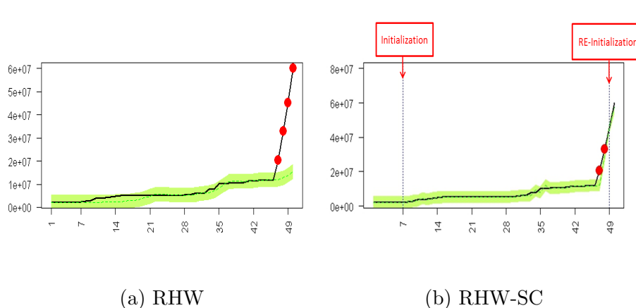
Figure 4: An industrial time series with a structural change
