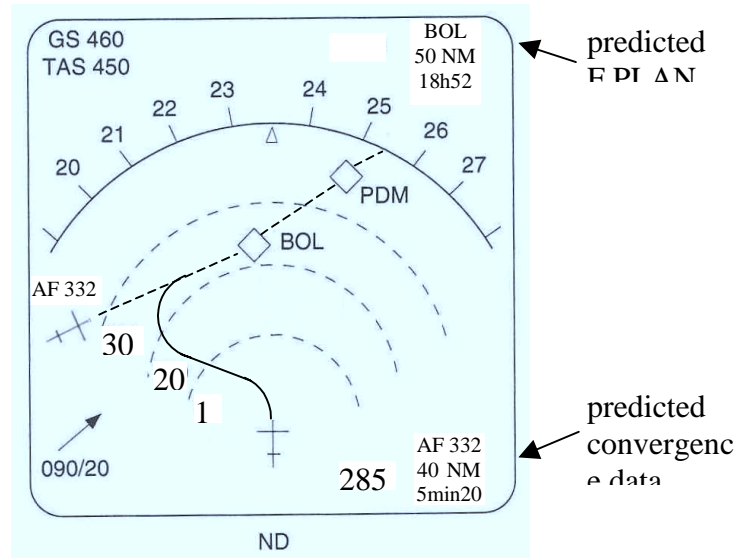
Figure 7. Presentation of a proposed or planned convergence maneuver to the pilot.
