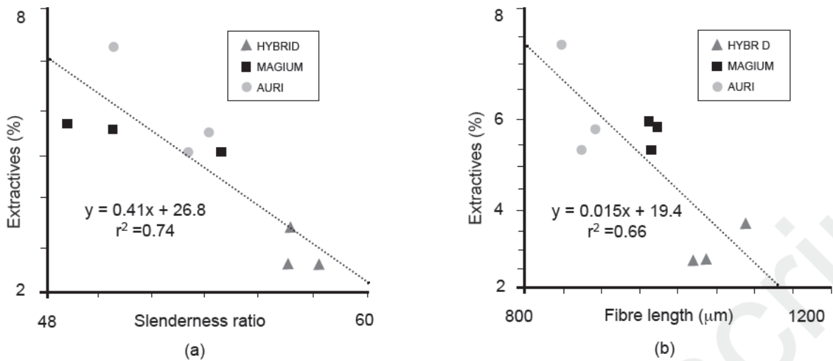
Figure 3 Relationship between extractives content and anatomical properties in acacias: (a) slenderness ratio and (b) fibre length
