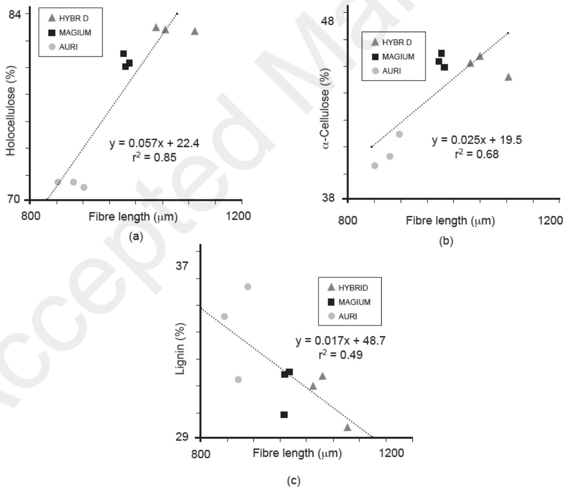
Figure 2 Relationships between chemical compositions and fibre length in acacias: (a) holocellulose, (b) \alpha -cellulose and (c) lignin content
