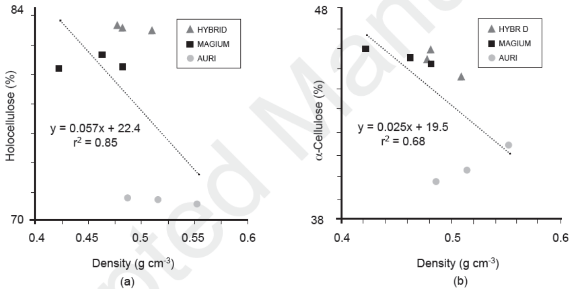
Figure 4 Relationships between chemical compositions and density in acacias: (a) holocellulose and (b) \alpha -cellulose
