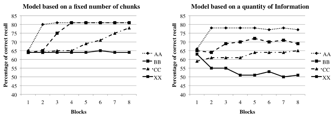
Figure 6: Percentage of correct recall for all blocks of 8 sequences, for each kind of stimuli. Model based on a fixed number of chunks is on the left side. Model based on a quantity of information is on the right side.
