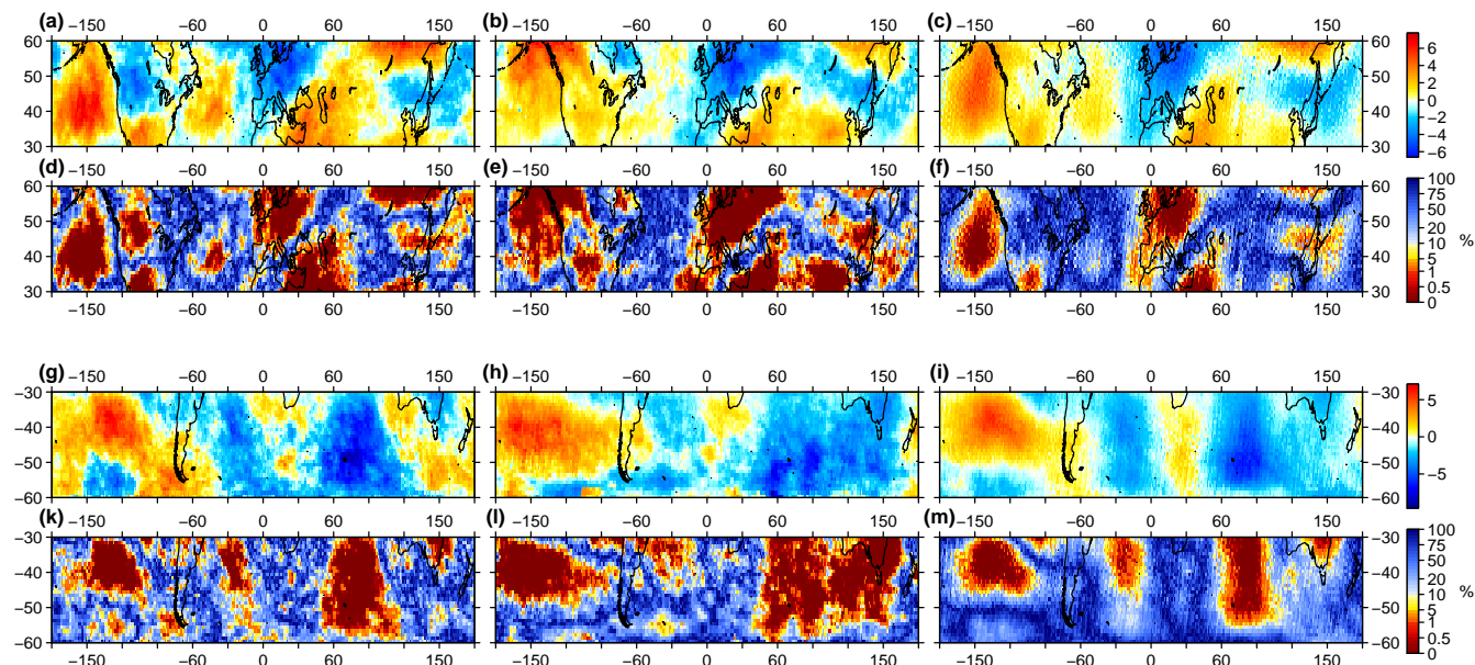
Fig. 2. Pointwise regression coefficient estimates (in \text{DU}(\text{unit ENSO})^{-1} ) for the El Niño/Southern Oscillation for (a) EHOs, (b) ELOs, and (c) mean values of total ozone during winter (DJF) at 30^\circ\text{N} to 60^\circ\text{N} ; (d)–(f) show the p -values of pointwise significance tests for the estimates in (a)–(c). (g)–(m) as (a)–(f) but during winter (JJA) at 30^\circ\text{S} to 60^\circ\text{S} . An augmented version of this figure including standard errors for all coefficient estimates is provided in Fig. S2.
