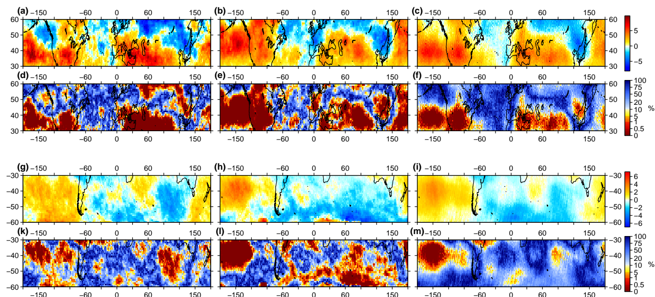
Fig. 3. Pointwise regression coefficient estimates (in \text{DU}(\text{unit ENSO})^{-1} ) for the El Niño/Southern Oscillation for (a) EHOs, (b) ELOs, and (c) mean values of total ozone during spring (MAM) at 30^\circ\text{N} to 60^\circ\text{N} ; (d)–(f) show the p -values of pointwise significance tests for the estimates in (a)–(c). (g)–(m) as (a)–(f) but during spring (SON) at 30^\circ\text{S} to 60^\circ\text{S} . An augmented version of this figure including standard errors for all coefficient estimates is provided in Fig. S3.
