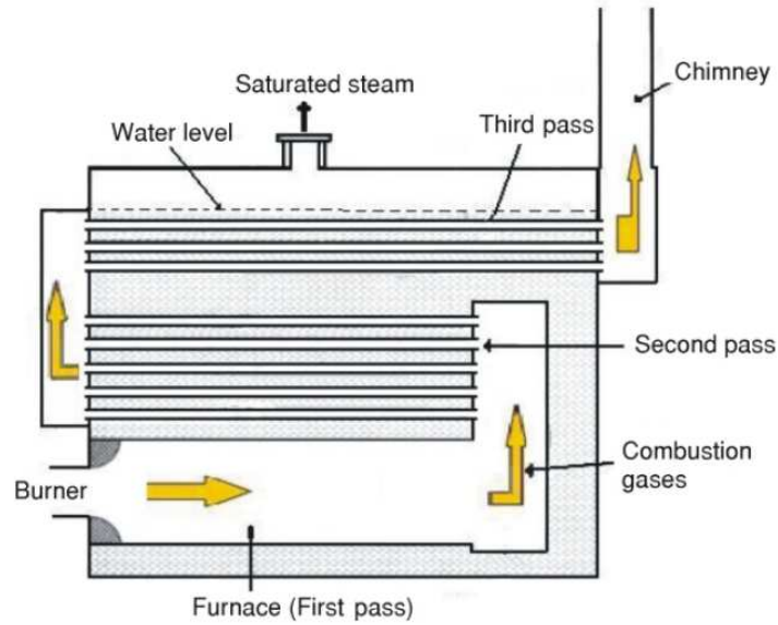
Figure 2. Schematic representation of a typical three-pass fire-tube boiler [29]
