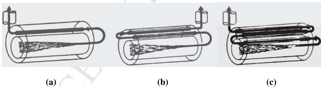
Figure 1. Basic gas flow patterns of a fire-tube (a) two-pass; (b) three-pass; (c) four-pass
