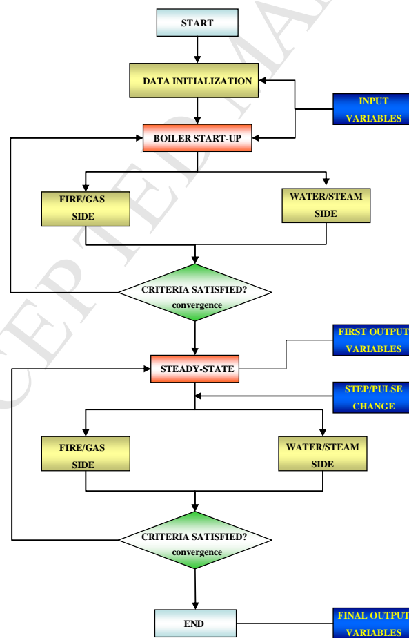
Figure 6. Overall calculation scheme of the complete model
