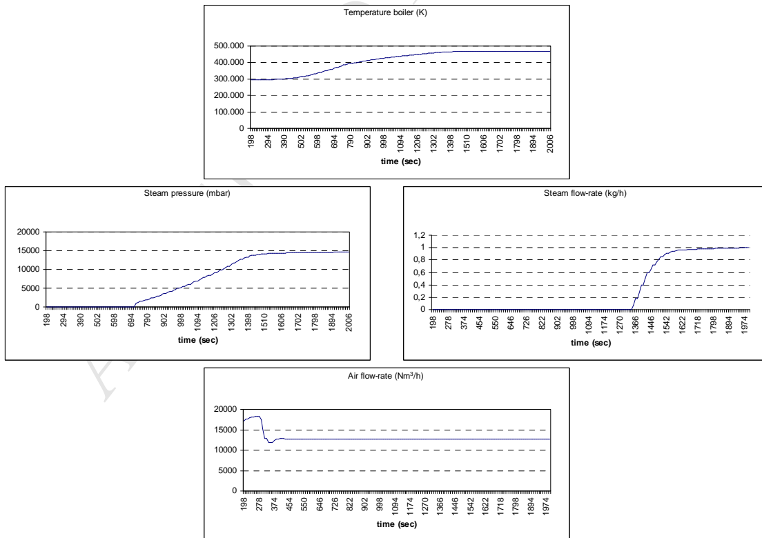
Figure 10. Dynamic behaviour of the boiler during the start-up initiated at t=0
