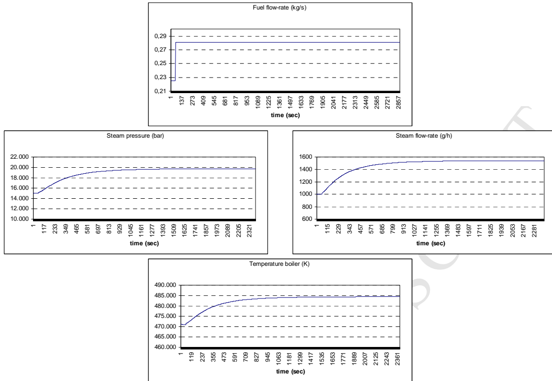
Figure 9. Dynamic behaviour of the boiler under a step in fuel flow-rate from 0.22 to 0.28 kg/s
