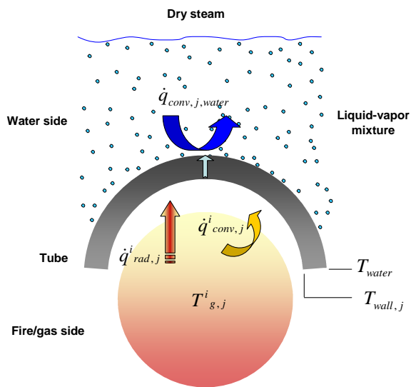
Figure 4. Schematic heat transfer phenomena occurring within a fire-tube boiler (under the water or phase -)
