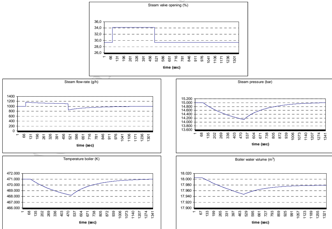
Figure 8. Dynamic behaviour of the boiler under a pulse in steam valve opening from 29.2 to 34.3% and back to 29.2%
