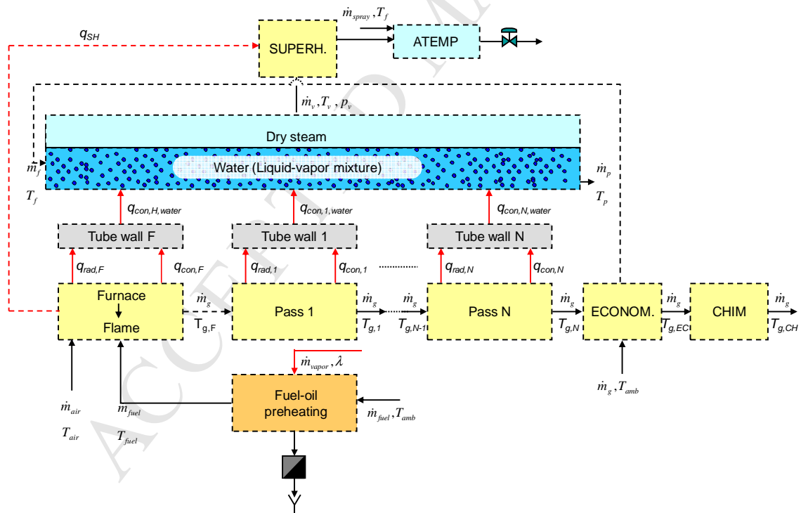
Figure 3. Scheme for the modeling of a fire-tube boiler
