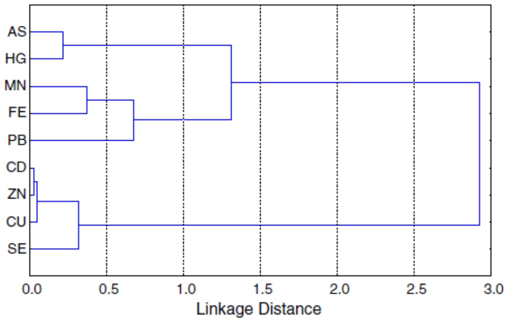
Tree Diagram for 9 Variables Ward's method 1-Pearson r
