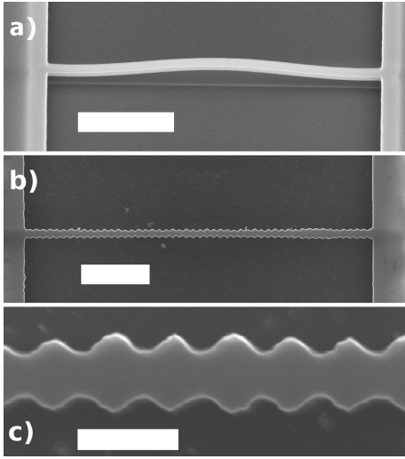
FIG. 1: SEM images of the straight a) and the corrugated b) nanowires; c) corresponds to the top view of the corrugated nanowire. The scale bars correspond to a) 2 \mu\text{m} , b) 2 \mu\text{m} and c) 300 \text{ nm} .
