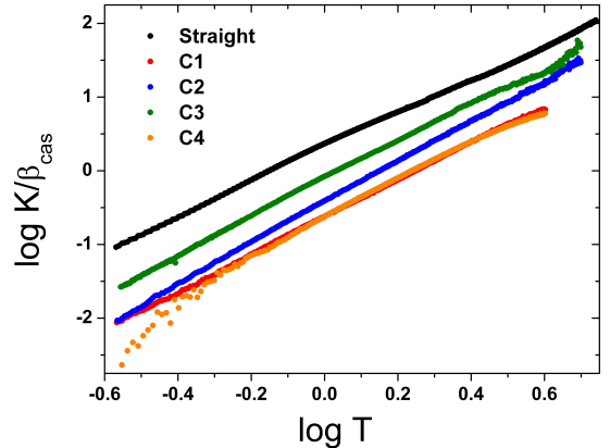
FIG. 3: (colour online) Log-log plot of the normalized thermal conductance of the straight and four corrugated nanowires versus the temperature. The normalization coefficient \beta_{Cas} corresponds to the Casimir limit value of the thermal conductance at 1 K.
