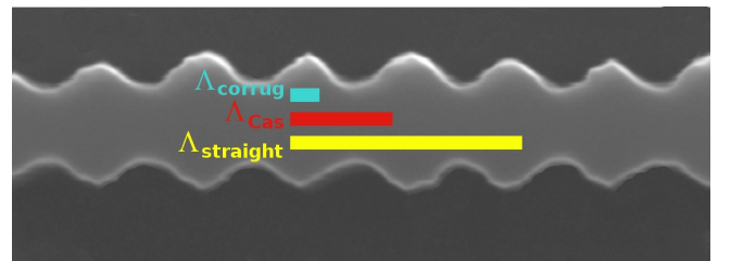
FIG. 4: (colour online) The Casimir MFP ( \Lambda_{Cas} = 220\text{nm} ), the effective MFP in the straight nanowire ( \Lambda_{straight} = 454\text{nm} ) and the corrugated nanowire C1 ( \Lambda_{corrug} = 57\text{nm} ) are compared to the actual geometry of the corrugated nanowire.
