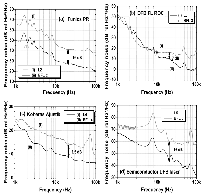
Fig. 5. Frequency noise spectra of (i) pump source (ii) Stokes component for different pump laser sources; namely (a) external cavity Tunics-PR, (b) distributed feedback fiber laser ROC (c) Koheras Ajustik and (d) distributed feedback semiconductor laser.
