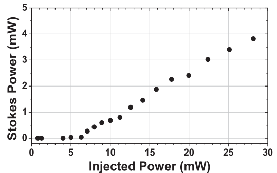
Fig. 2. BFL output power as a function of injected pump power.
