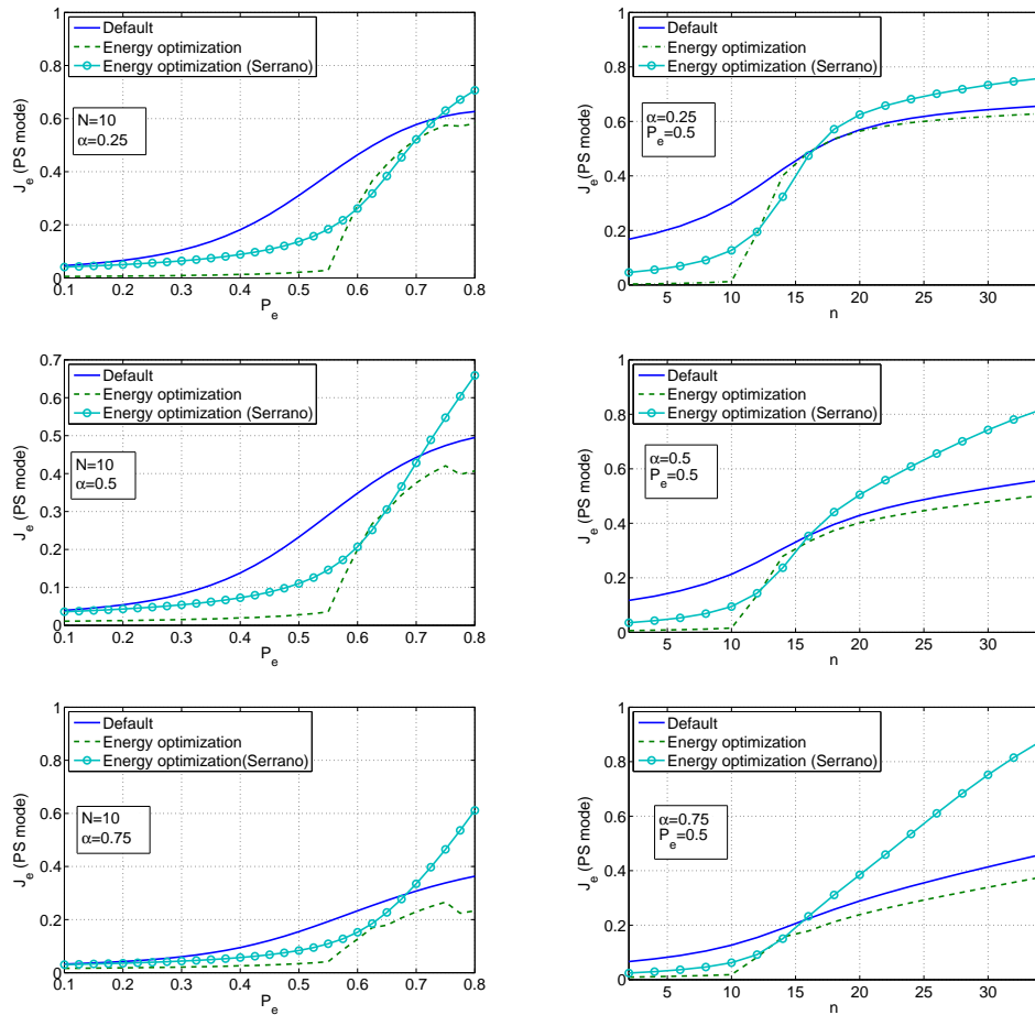
Figure 17: Joint cost function obtained with different configuration mechanisms for various values of \alpha and stations operating in PS mode. Plots on the left column show the results for 10 stations and variable packet error probabilities. Plots on the right column show the results for various numbers of stations and fixed packet error probability.
