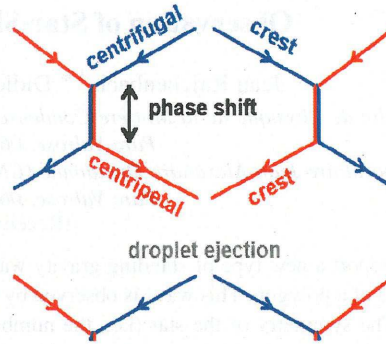
FIG. 2 (color online). Same experimental conditions as in Fig. 1. The present spatiotemporal diagram corresponds to the time evolution of the line of pixels passing through the center of the vessel. The line of pixels is plotted horizontally, and the time here is downward. This plot allows us to visualize the motion of the contrapropagative crests, and to measure the a phase delay when crossing. For these experimental conditions, the phase delay is equal to 0.05 s.
