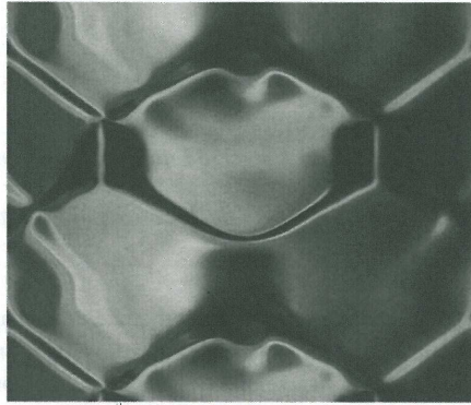
FIG. 2 (color online). Same experimental conditions as in Fig. 1. The present spatiotemporal diagram corresponds to the time evolution of the line of pixels passing through the center of the vessel. The line of pixels is plotted horizontally, and the time here is downward. This plot allows us to visualize the motion of the contrapropagative crests, and to measure the a phase delay when crossing. For these experimental conditions, the phase delay is equal to 0.05 s.
