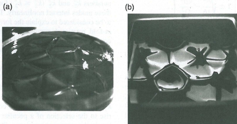
FIG. 5. For identical filling level, vibration parameters, and forcing history, the wave pattern is independent of the container shape and size. (a) In a cylindrical container of radius 17 cm, we observe a tiling of star-shaped waves. (b) In a square container (17 cm \times 17 cm), we observe analogue patterns. Note that here adjacent pentagons and five-branched stars oscillate with a phase shift of \pi . This is an example of the possible solutions issued from the subharmonic instability.
