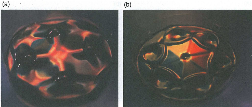
FIG. 6 (color online). Stars and polygonal waves with other symmetries can be observed with other vibration parameters or filling levels. (a) Symmetry of 4th order (filling level 8 mm, vibration amplitude 2.40 mm, \Omega/2\pi = 12 Hz). (b) Symmetry of 6th order (filling level 8 mm, vibration amplitude 2.90 mm, \Omega/2\pi = 12 Hz).
